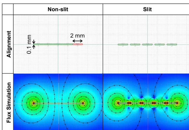
Figure 6. Analysis of magnetic flux for two designs of samples. Slit-designed FluxPaper (right) has a strong magnetic field between slits.
