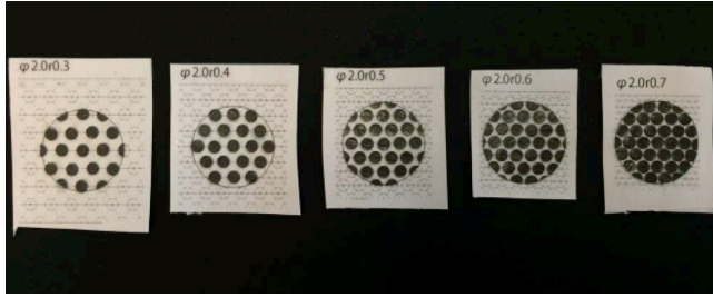
Figure 8. Different area ratio (30%, 40%, 50%, 60%, 70%) of magnetic layer on samples.
