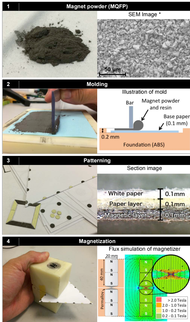
Figure 4. Laboratory-level production process. (*SEM image is cited from Magnequench's document [16].)
