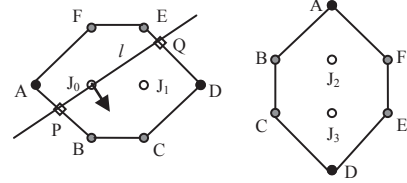
Fig. 3. On-block interpolation layout
